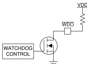
图 8-3. \overline{WDO} Open-Drain Configuration
